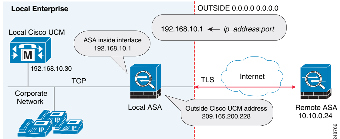
Figure 21-9 Example for Configuring Off Path Signaling in an Off Path Deployment
